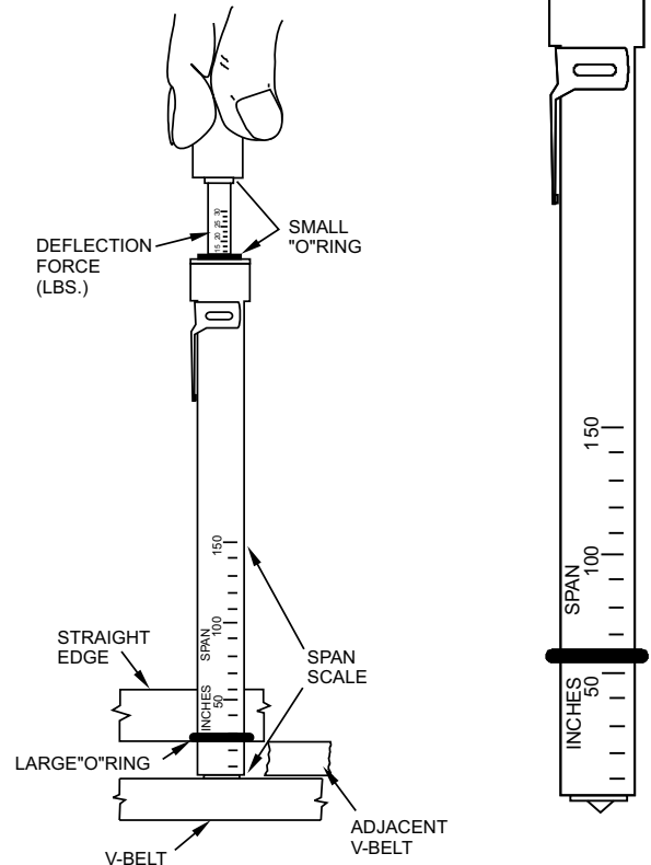
Part Number: "Belt Tension Checker"
